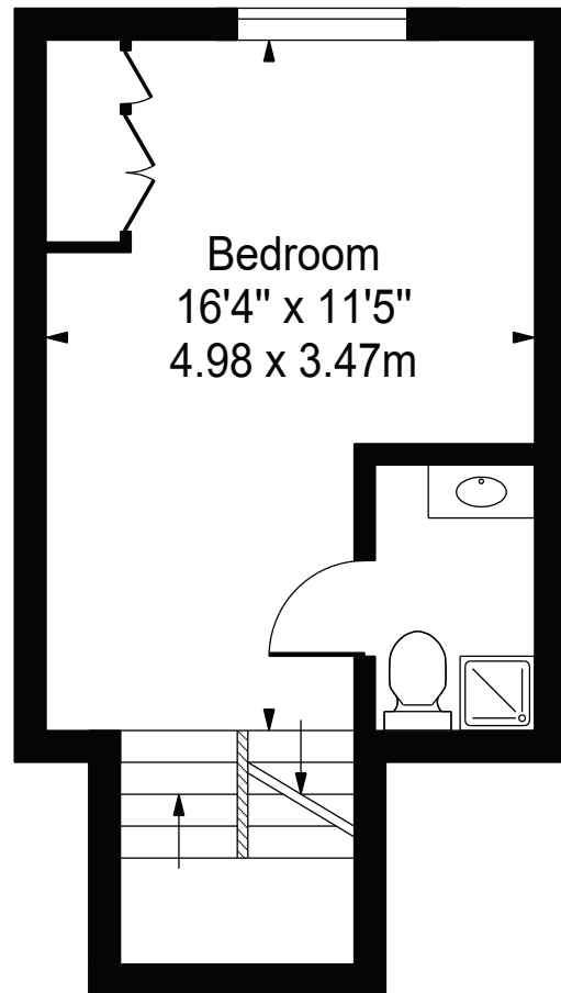
Forth Floor
