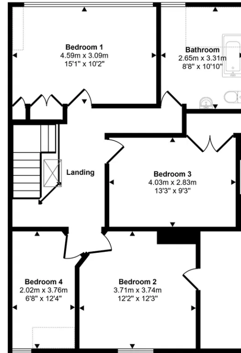
First Floor Approx 81 sq m / 873 sq ft
