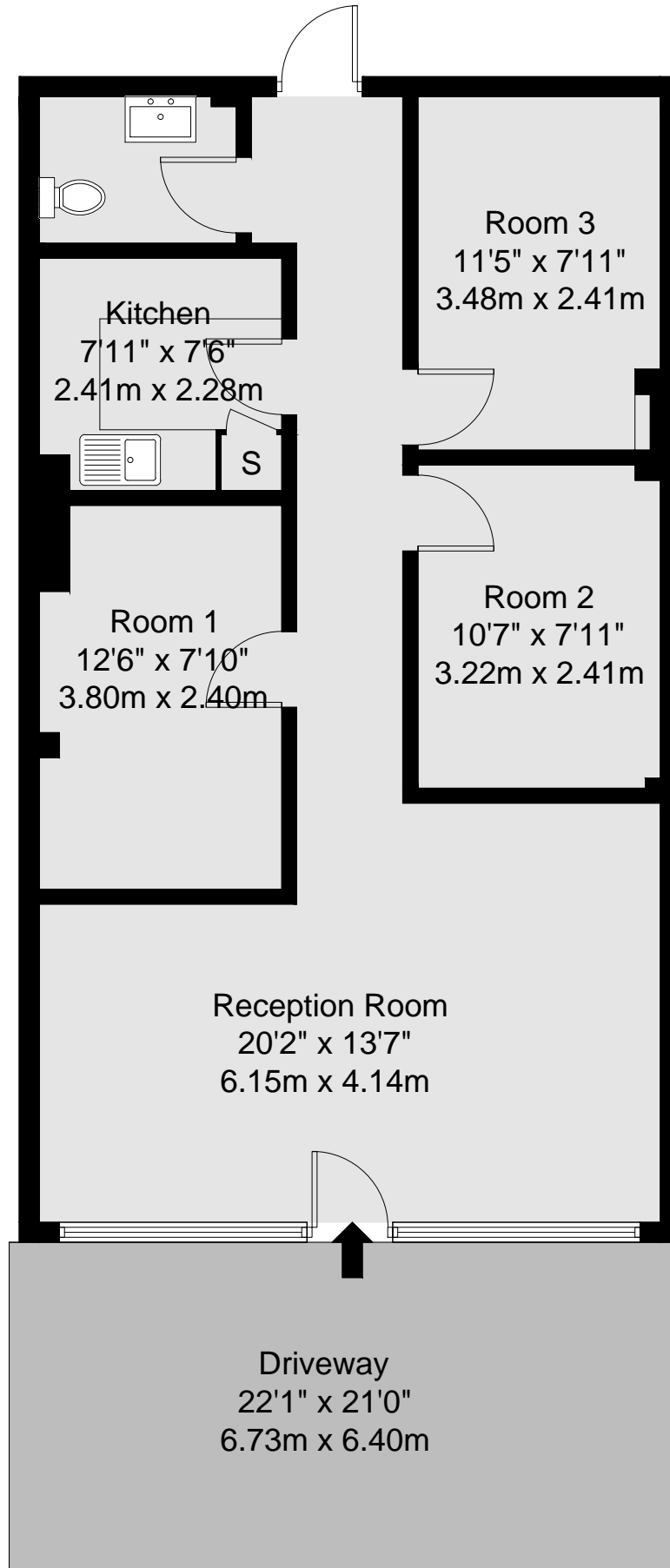
Ground Floor
