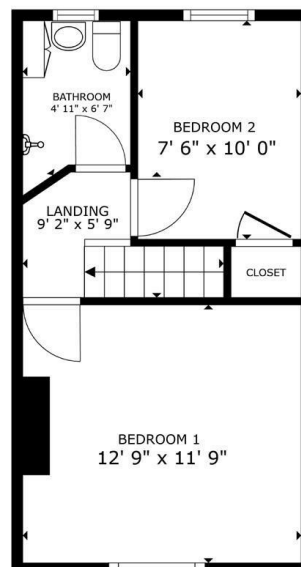
FLOOR 2
