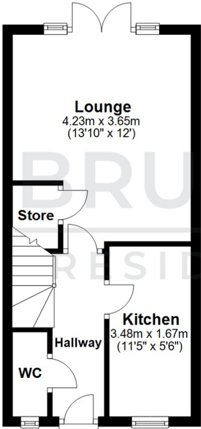
Ground Floor Approx. 28.4 sq. metres (305.7 sq. feet)
