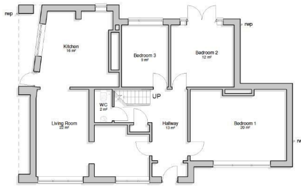
Ground Floor 1 : 100
