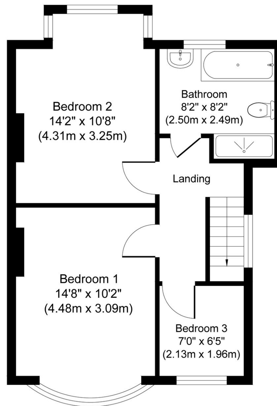
First Floor Approximate Floor Area 478 sq. ft (44.38 sq. m)
